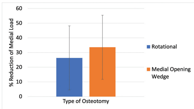
Fig. 11 Percentage reduction of load through the medial compartment for external rotational constructs compared to opening wedge constructs. This graph demonstrates all rotational constructs compared to all opening wedge constructs (including all osteotomy directions, levels, and angles).
